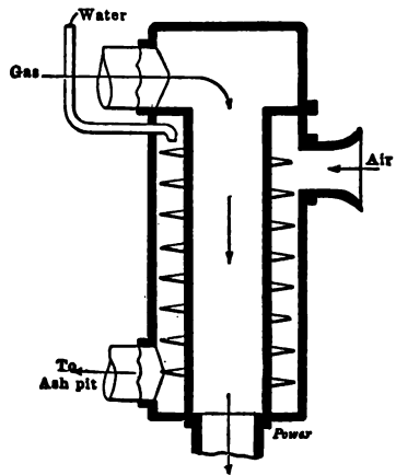
FIG. 86.—Combined Vaporizer and Economizer.
